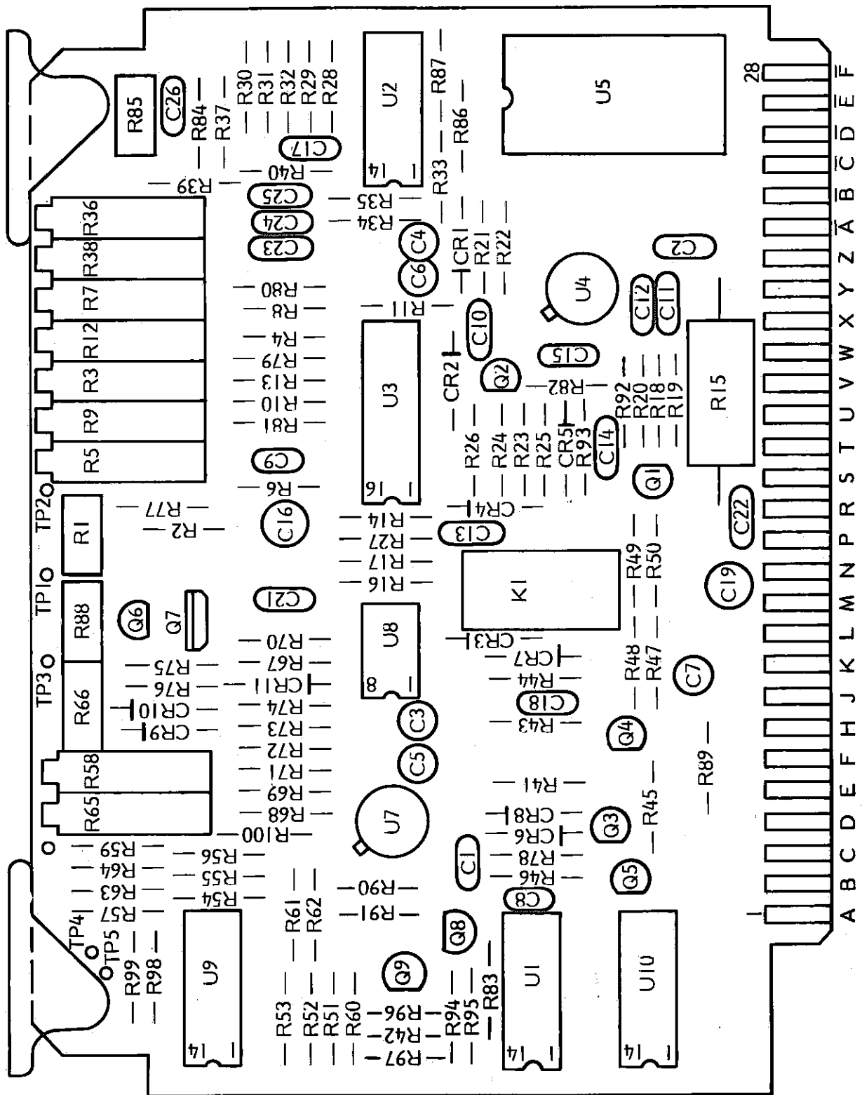
YIG Driver Parts Locator Diagram
